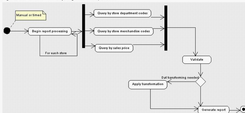
Figure 3.0.1 Run Nightly Reports
