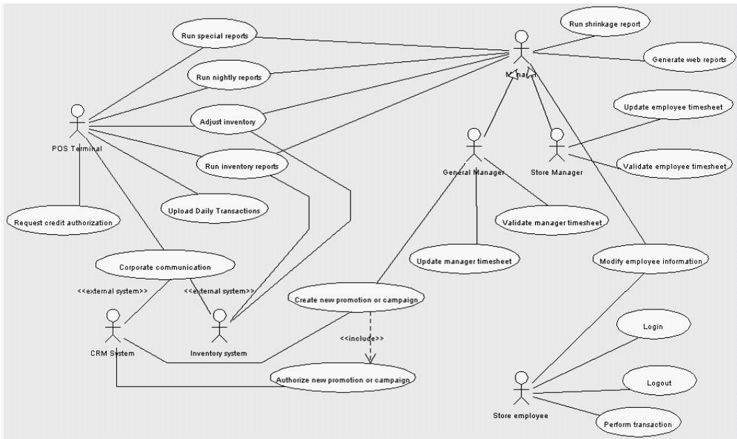
Use Case Diagram 2.0.1 Store POS Application
