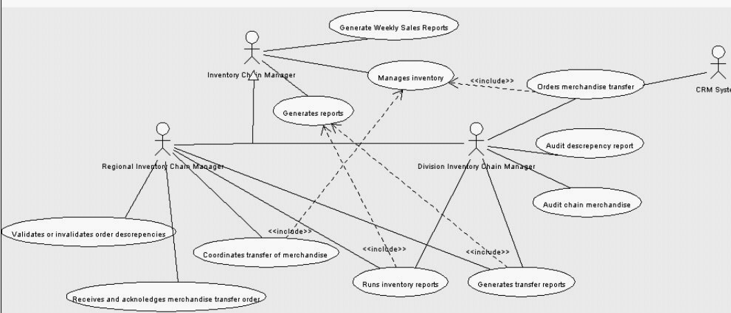
Use Case Diagram 2.0.1 Store POS Application
