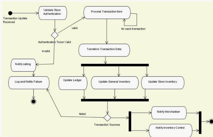
Figure 3.0.4 Daily Transaction Upload
